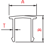
PSP2997 Reinforcement Cap Profile
