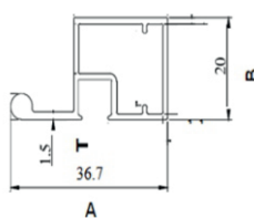
PSPMOS05 MOSQUITO SHUTTER SERIES(MOS)
