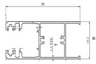
PSP3603 SHUTTER SECTION
