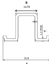
PSP3608 LAMINATED GLASS CLIP
