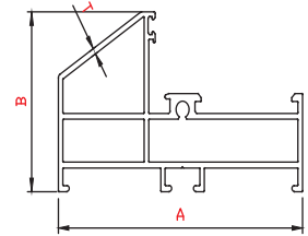
PSP5003 50mm Casement Window Tapper Frame
