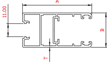
PSP2925 SGU Light Shutter For Mosquito only
