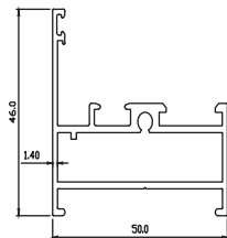
PSP5004 50mm Casement Frame
