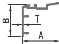
PSP2791 Interlocking Plate
