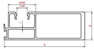
PSP2994 29 mm Sleek Reinforcement Interlock
