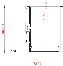
PSP5005 50mm Door Frame
