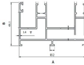
PSP3602 2 TRACK WITH LEG
