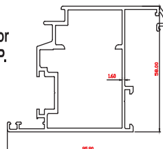
PSP5023 50mm Door Shutter
