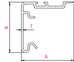
PSP2991 Interlock
