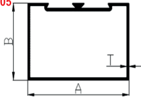
PSP1001 PSP1005 SINGLE PARTITION
