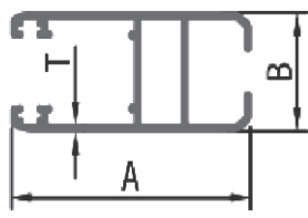
PSP2721 Handle
