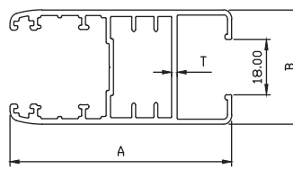
Shutter for Single Point Locking OR Champion Plus Laminated Glass
