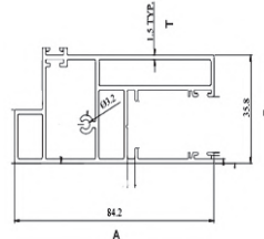
PSP3605 TRACK SHUTTER
