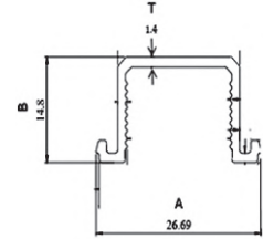
PSP3606 LAMINATED GLASS CLIP
