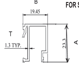
SINGLE GLASS BEAD FOR SHUTTER
