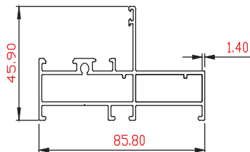
PSP 50mm Casement Window Frame
