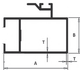
PSP1131 50X25 INTERLOCK
