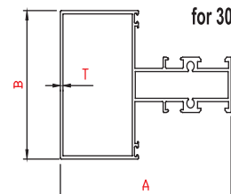
PSP5051 50mm Casement Window Mullion for 30mm Glass
