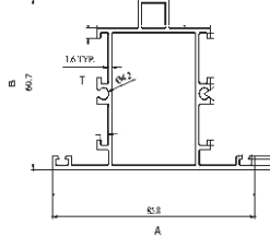
INVERSION SECTION
