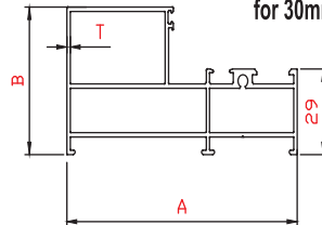
PSP5002 50mm Casement Window Frame for 30mm Glass
