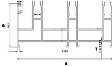
PSP3601 3 TRACK WITH LEG
