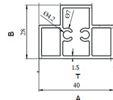
PSPMOS03 MOSQUITO SHUTTER SERIES(MOS)
