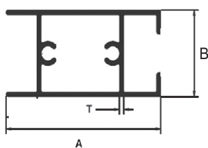
PSP1121 50X25 TOP BOTTOM
