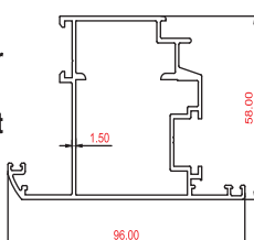
PSP5025 50mm Door Shutter
