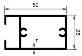
PSP1111 50X25 HANDLE
