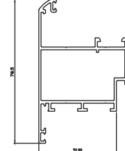
PSP5021 50mm Casement Shutter
