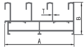
PSP2703 Four Track Sliding Series
