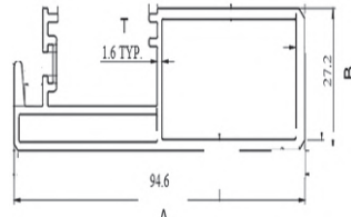
PSP3611 SLEEK INTERLOCK WITH REINFORCEMENT SECTION
