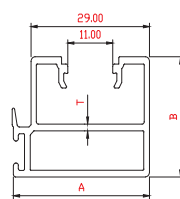
PSP2993 29 mm Sleek Interlock
