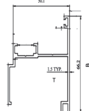
FLYING MULLION PROFILE
