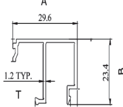
DGU GLASS BEAD FOR FIX
