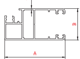
PSP2927 Mosquito Shutter
